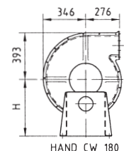
HAND CW 180
