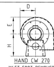
HAND CW 270 INLET FOOT REMOVED
