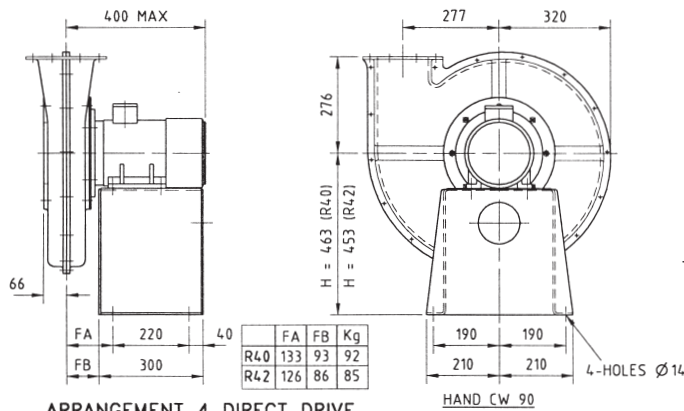
ARRANGEMENT 4 DIRECT DRIVE
