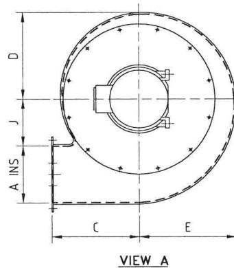
VIEW A
