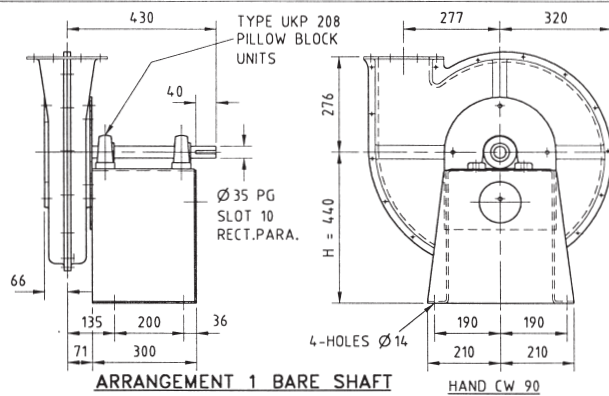
ARRANGEMENT 1 BARE SHAFT R40 FAN WEIGHT = 64 KG
