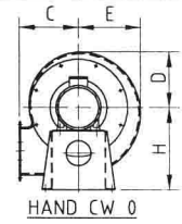
HAND CW 0
