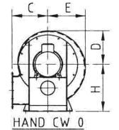
HAND CW 0
