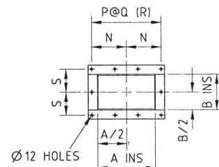
DISCHARGE FLANGE 40x5 FLAT
