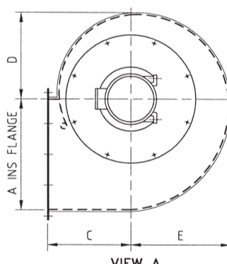
VIEW A
