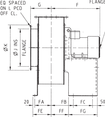
ARRANGEMENT 4 DIRECT DRIVE
