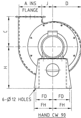
HAND CW 90
