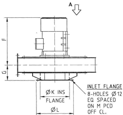
ARRANGEMENT 4F DIRECT DRIVE
